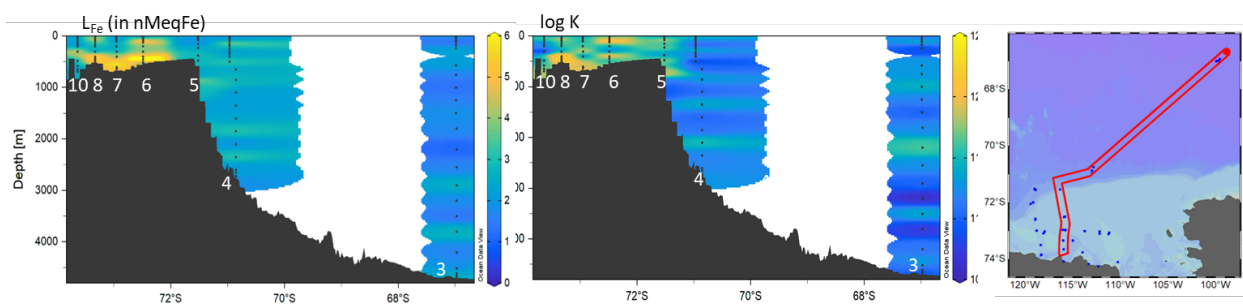
Figure 7. Iron-binding ligand characteristics (log K and L_{Fe} ) for Stations 3 to 10 analyzed at sea.
