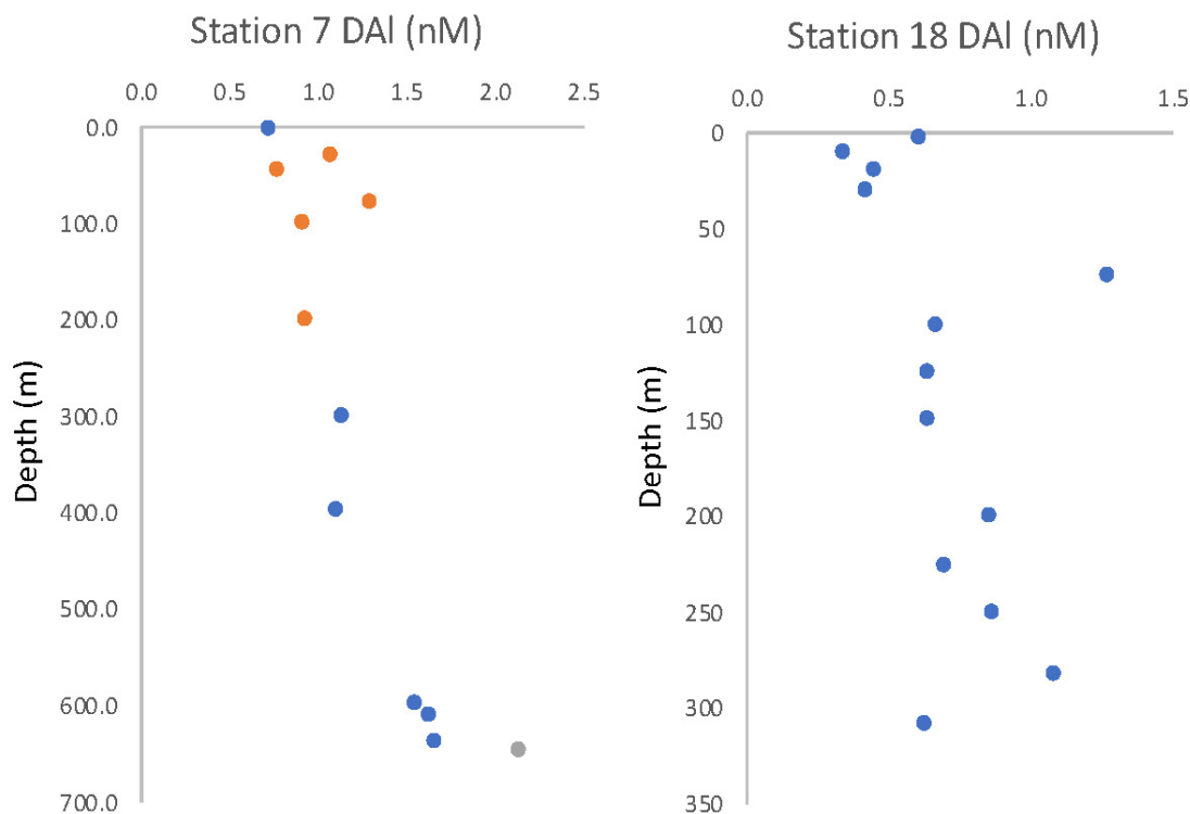
Figure 10. Dissolved Al concentration profiles from Station 7 in the central Dotson Trough (left panel) and Station 18 over Bear Ridge (right panel). For Station 7, the orange and blue symbols indicate samples taken from two separate GTC rosette casts, and the gray symbol indicates the multicorer Niskin-X sample.
