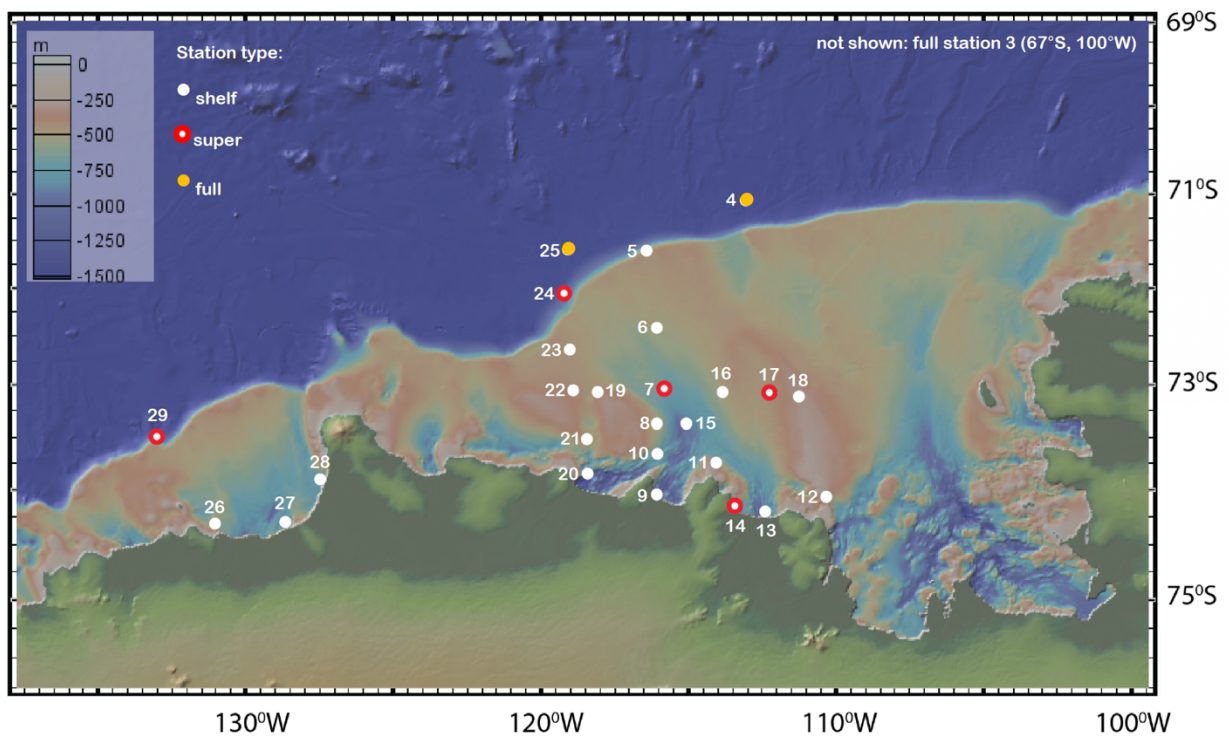
Bathymetric map of the Amundsen Sea showing GP17-ANT sampling stations
