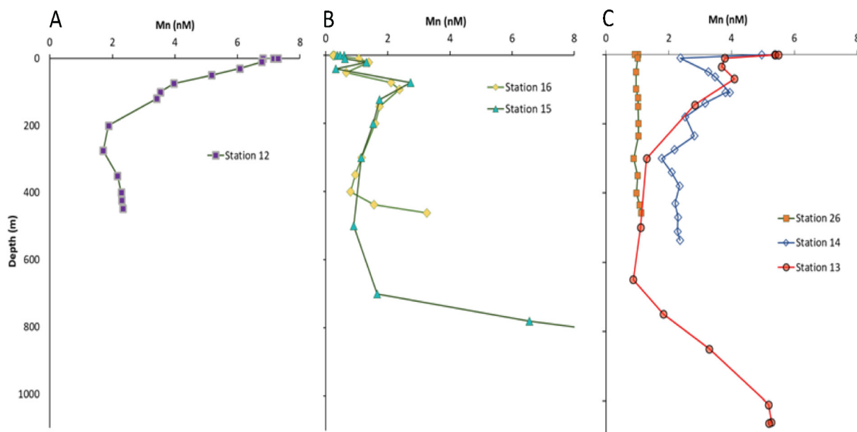
Figure 9. Dissolved Mn concentration profiles from (A). Station 12 on the inner shelf northeast of Bear Island (low biomass); (B). Stations 15 and 16 on the inner shelf in the Amundsen Sea Polynya (high biomass); and (C). Stations adjacent to ice shelves: Station 13 (Dotson inflow), Station 14 (Dotson outflow), and Station 26 (Getz-E outflow).
