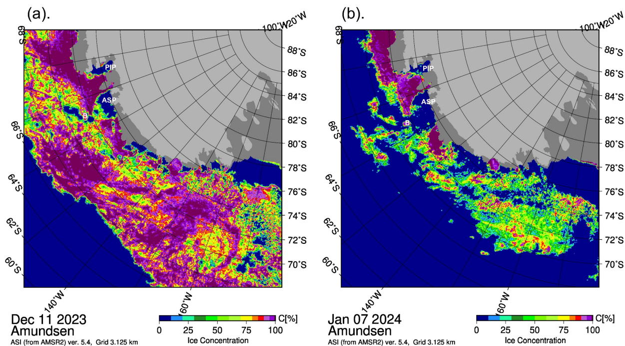
Figure 3. Maps showing sea-ice concentration (%) estimated from AMSR2 and AMSR-E satellite microwave data for (a) 11 December 2023, as we approached the Amundsen Sea shelf, and (b) 7 January 2024, as we began a transit west to sample our last few stations (Fig. 2). Shown are the Pine Island Polynya (PIP), Amundsen Sea Polynya (ASP), and iceberg B-22A (B). Note the heavy sea ice cover (purple) that prevented the ship's access to the Pine Island Polynya. Images: University of Bremen.
