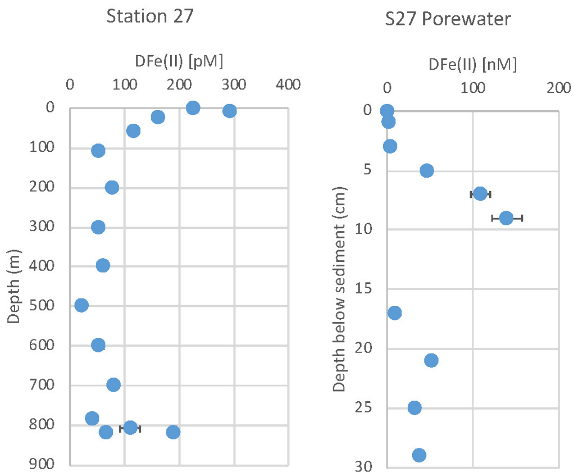
Figure 4. Vertical profiles of dissolved iron(II) concentrations in the water column (left) and sediment pore waters (right) from Station 27.
