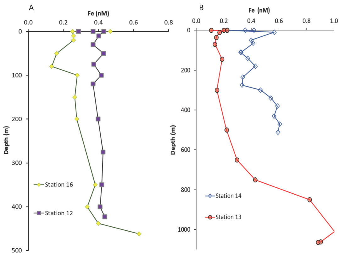
Figure 8. Dissolved Fe concentration profiles from (A). Stations 12 on the inner shelf northeast of Bear Island (low biomass) and 16 on the inner shelf in the Amundsen Sea Polynya (high biomass); and (B). sites adjacent to the Dotson Ice Shelf: Stations 13 (inflow) and 14 (outflow).
