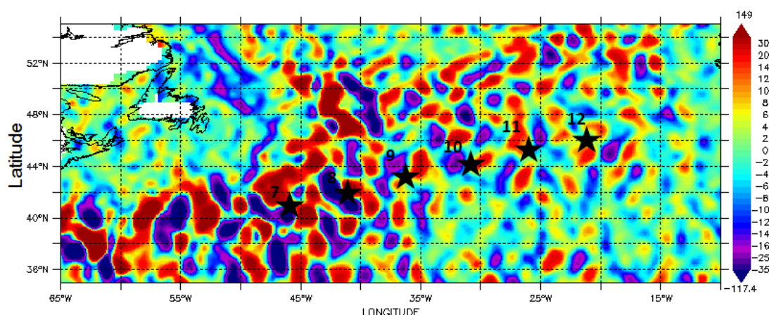
Figure 22. East component of the zonal geostrophic velocity in cm/s (7 August 2012 ). The figure shows the barotropic component of the geostrophic current, resulting from the altimetry data. The positive values (red) indicate a current from the west to the east and the negative values indicate a current from the east to the west. Stations 7 to 12 are plotted (dark stars). Source: http://las.aviso.oceanobs.com
